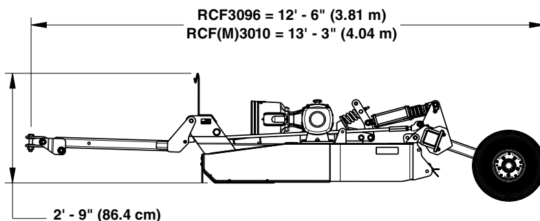
Pull-Type Rotary Cutter (RC3096 Shown)
