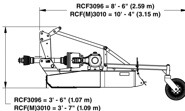
3-Point Mounted Rotary Cutter (RC3096 Shown)
