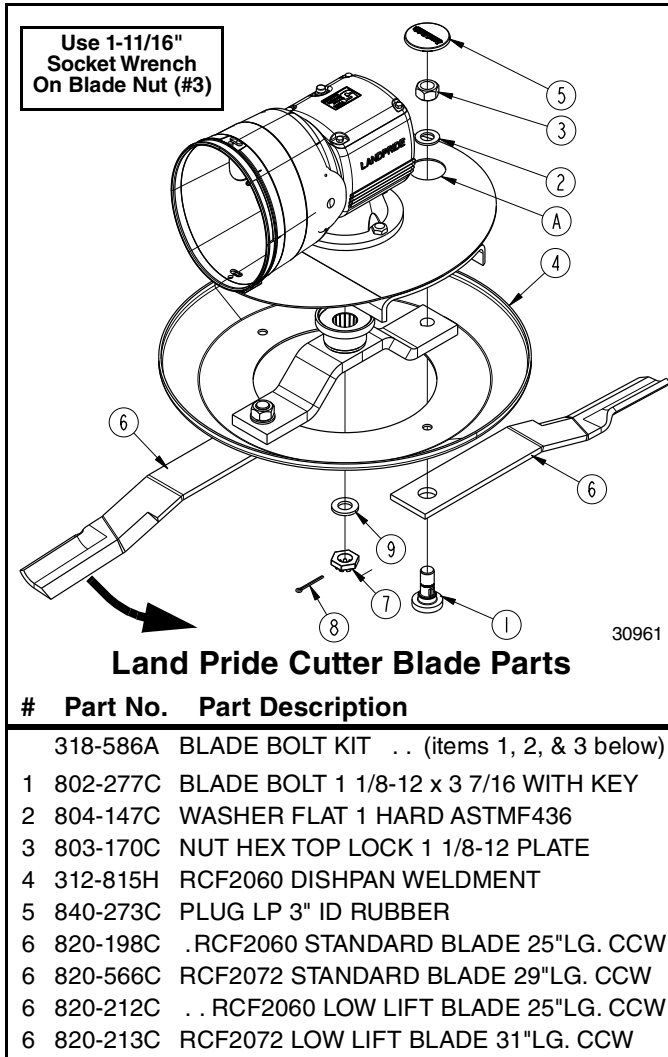
Cutter Blade Assembly (Counterclockwise Rotation) Figure 5-1
