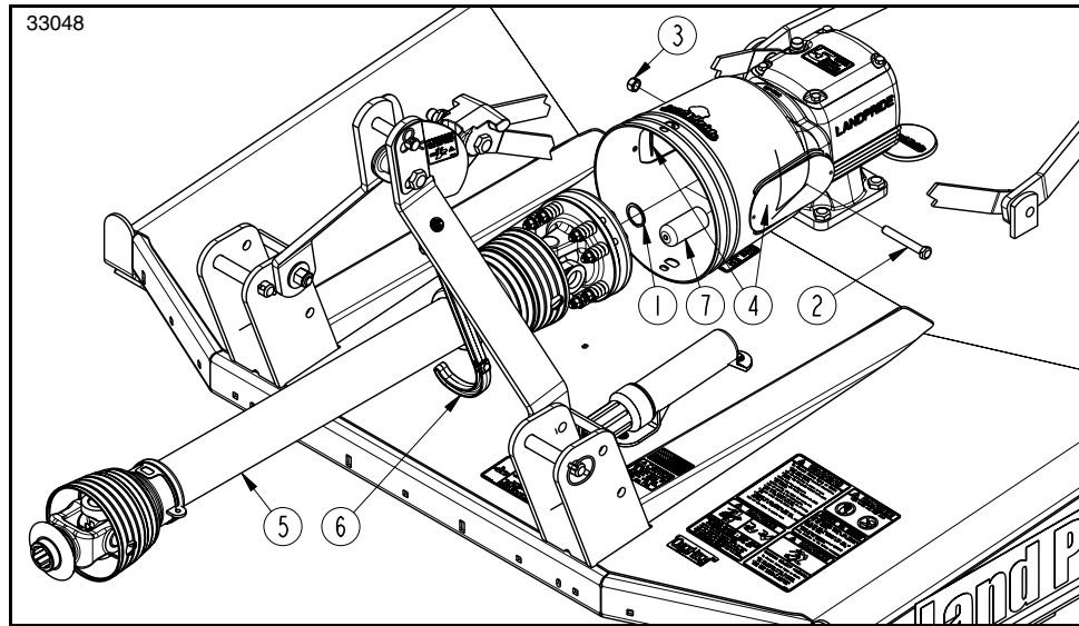
Driveline Installation Figure 1-3
