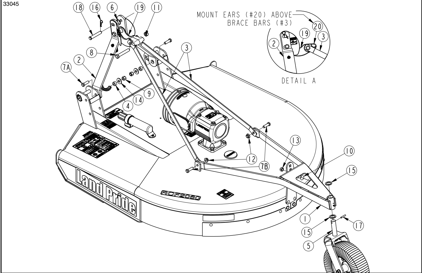
Hitch Assembly Figure 1-2
