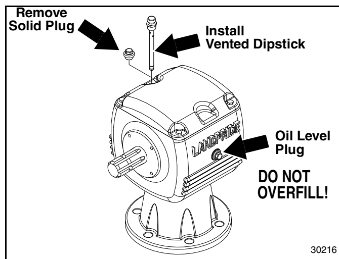
Gearbox Vented Dipstick Installation Figure 1-1
