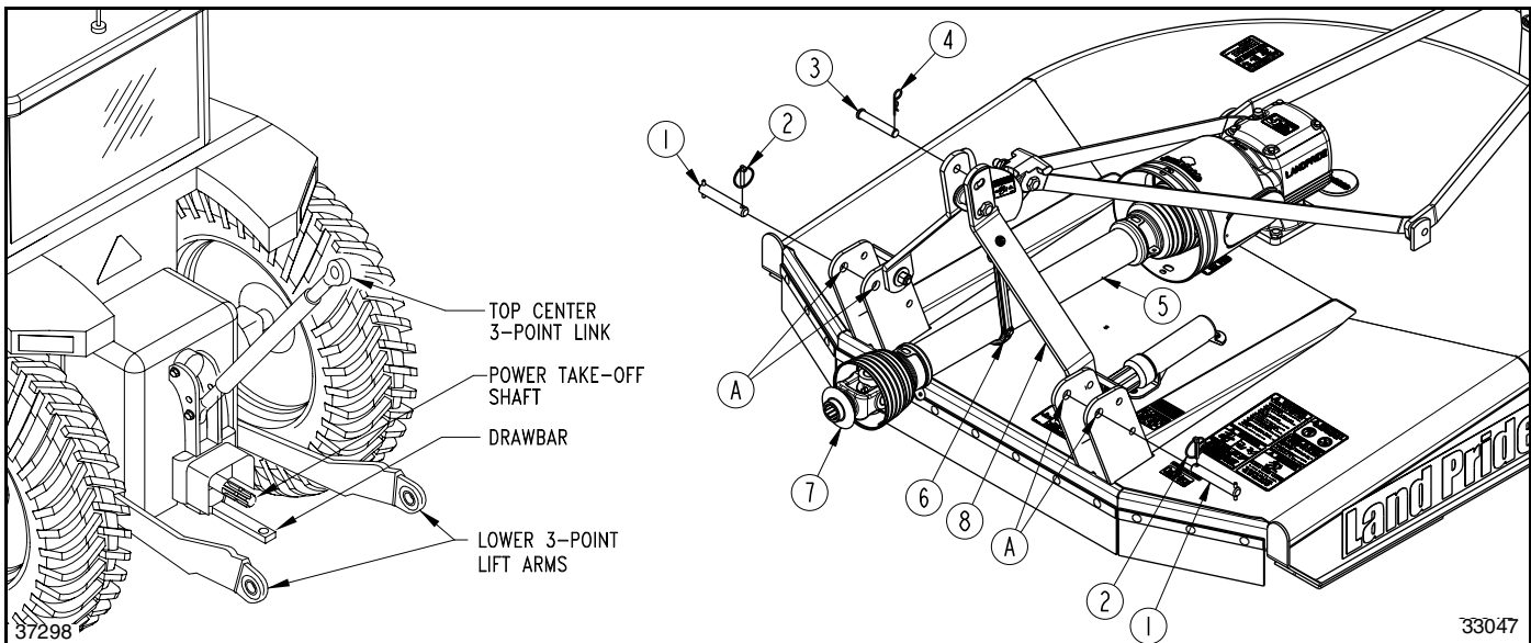
Tractor Hook-Up Figure 1-4
