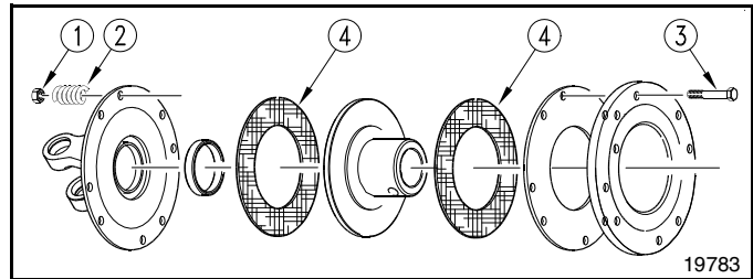
Clutch Assembly Figure 5-4
