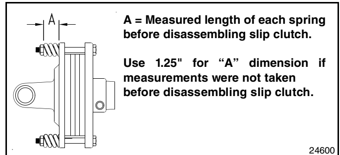
Clutch Adjustment Figure 5-6
