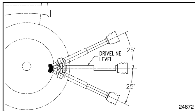
Maximum Driveline Movement During Operation Figure 1-8
