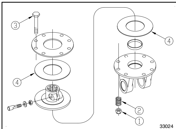
Clutch Disassembly Figure 5-5
