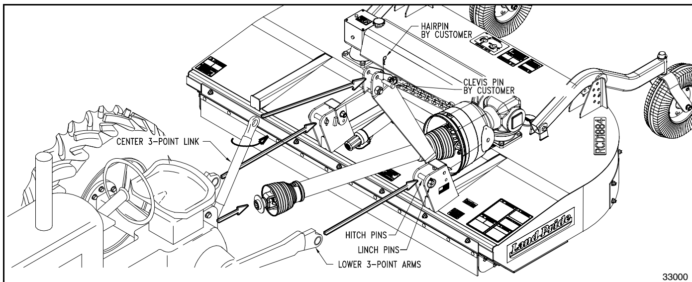
Tractor Hook-Up Figure 1-3
