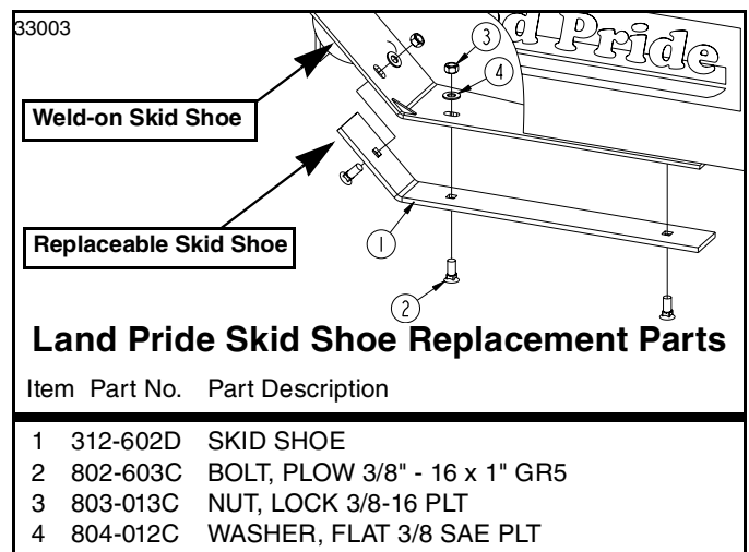
Skid Shoe Accessory Figure 5-7
