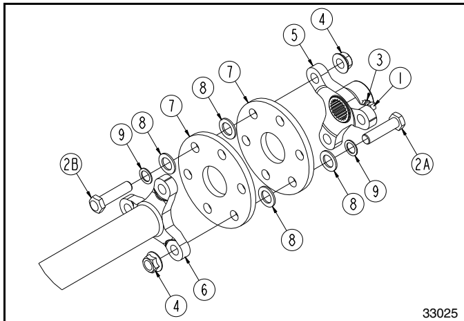
Flex Coupler Assembly Figure 5-3
