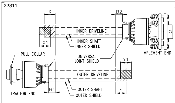
Driveline Shortening Figure 1-6
