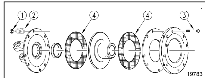
Clutch Disassembly Figure 4-4
