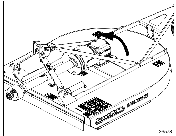
Counterclockwise Blade Rotation Figure 4-2
