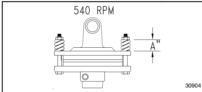
Clutch Adjustment Figure 4-5
