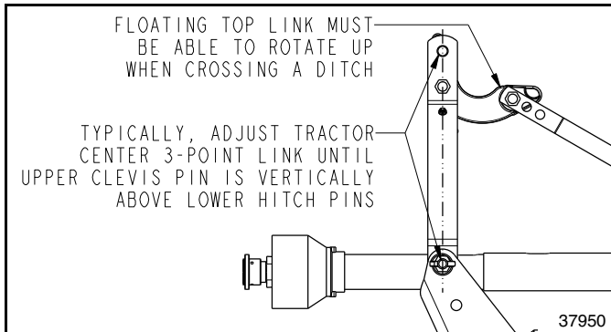
Deck Leveling Figure 3-3
