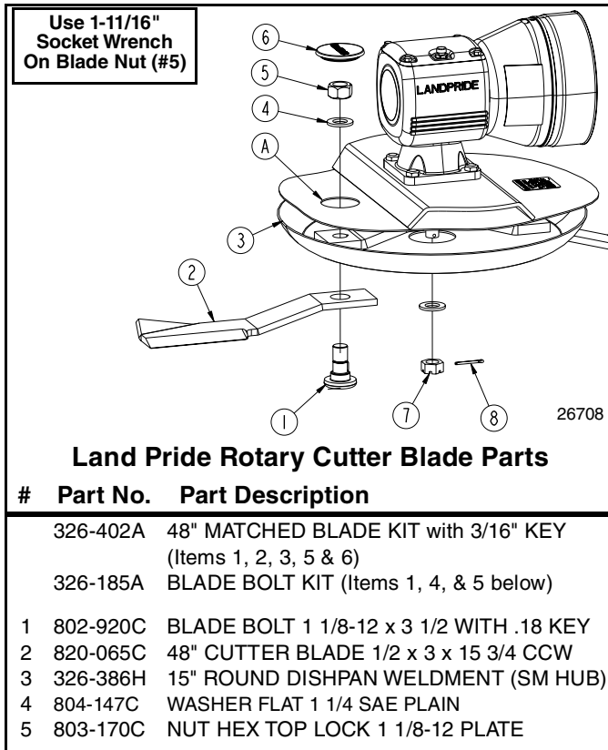
Cutter Blade Assembly Figure 4-1
