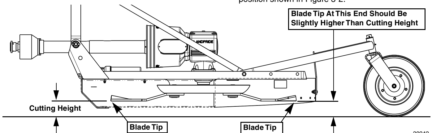
Cutting Height Figure 3-2
