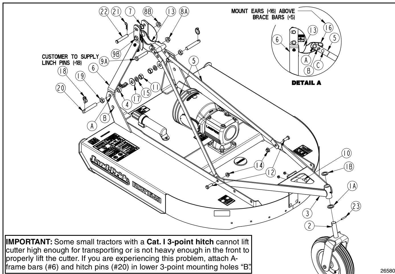
Dealer Assembly Figure 1-1
