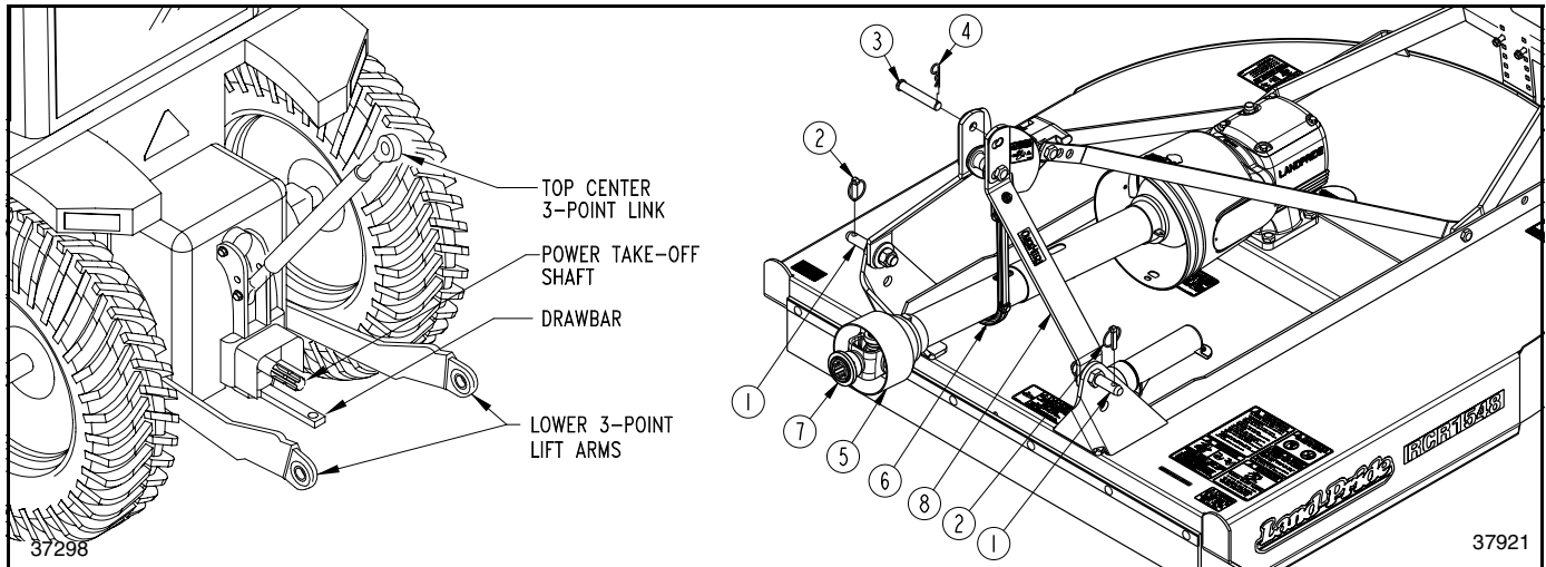
Tractor Hook-Up Figure 1-4
