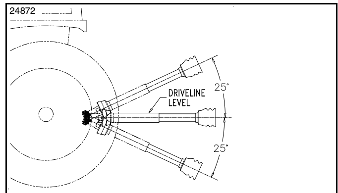
Maximum Driveline Movement During Operation Figure 1-7
